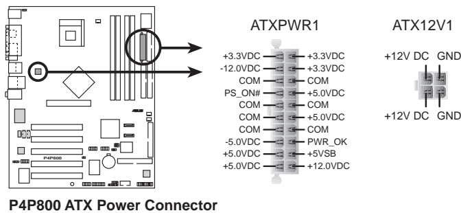
P4P800 ATX Power Connector
