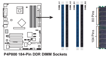
P4P800 184-Pin DDR DIMM Sockets
