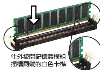
P4P800 184-Pin DDR DIMM Sockets
