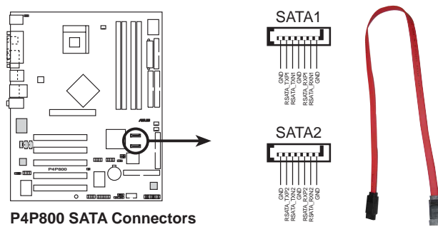
P4P800 SATA Connectors
