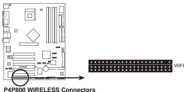
P4P800 WIRELESS Connectors
