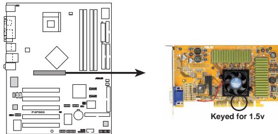
P4P800 Accelerated Graphics Port (AGP)
